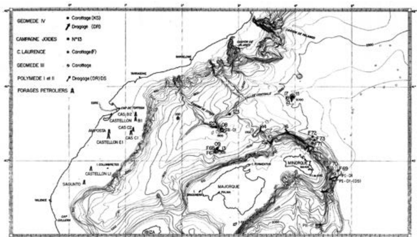
Figure 3. Detailed bathymetry of the Balearic Promontory in the Western Mediterranean Sea. Location of main 1975 known cores and marine campaigns. From Bourrouilh and Mauffret, 1975.
